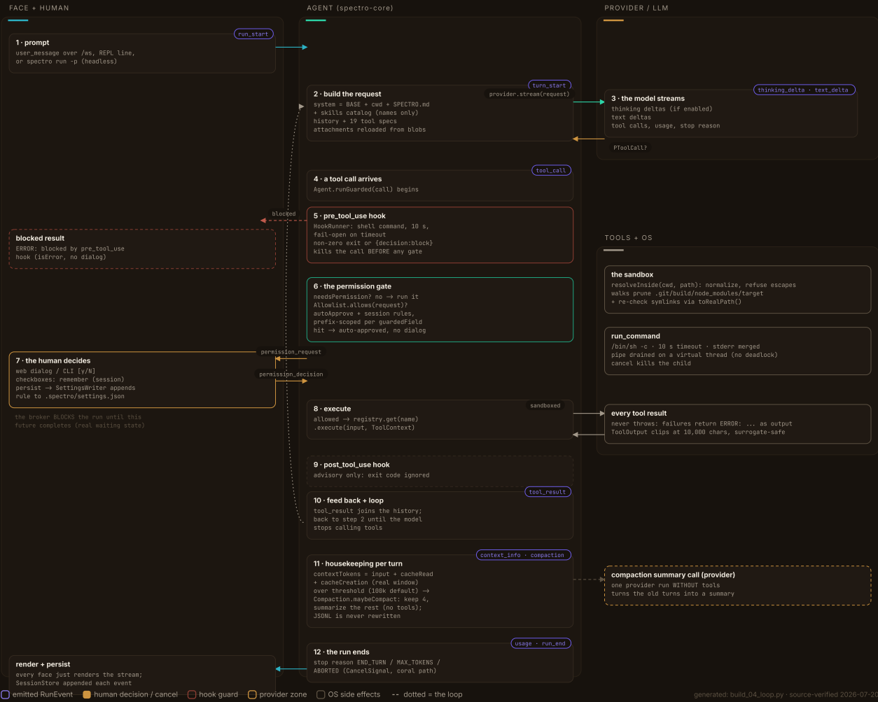
Diagram 04 — one turn as a swimlane: request build, streaming, the pre_tool_use hook, allowlist and human gate, sandboxed execution, the feedback loop into the next turn, compaction and run end.
